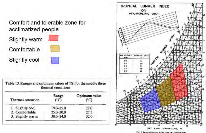
Fig. 10. Tropical Summer Index (TSI) - thermal zones on psychrometric chart [27]
